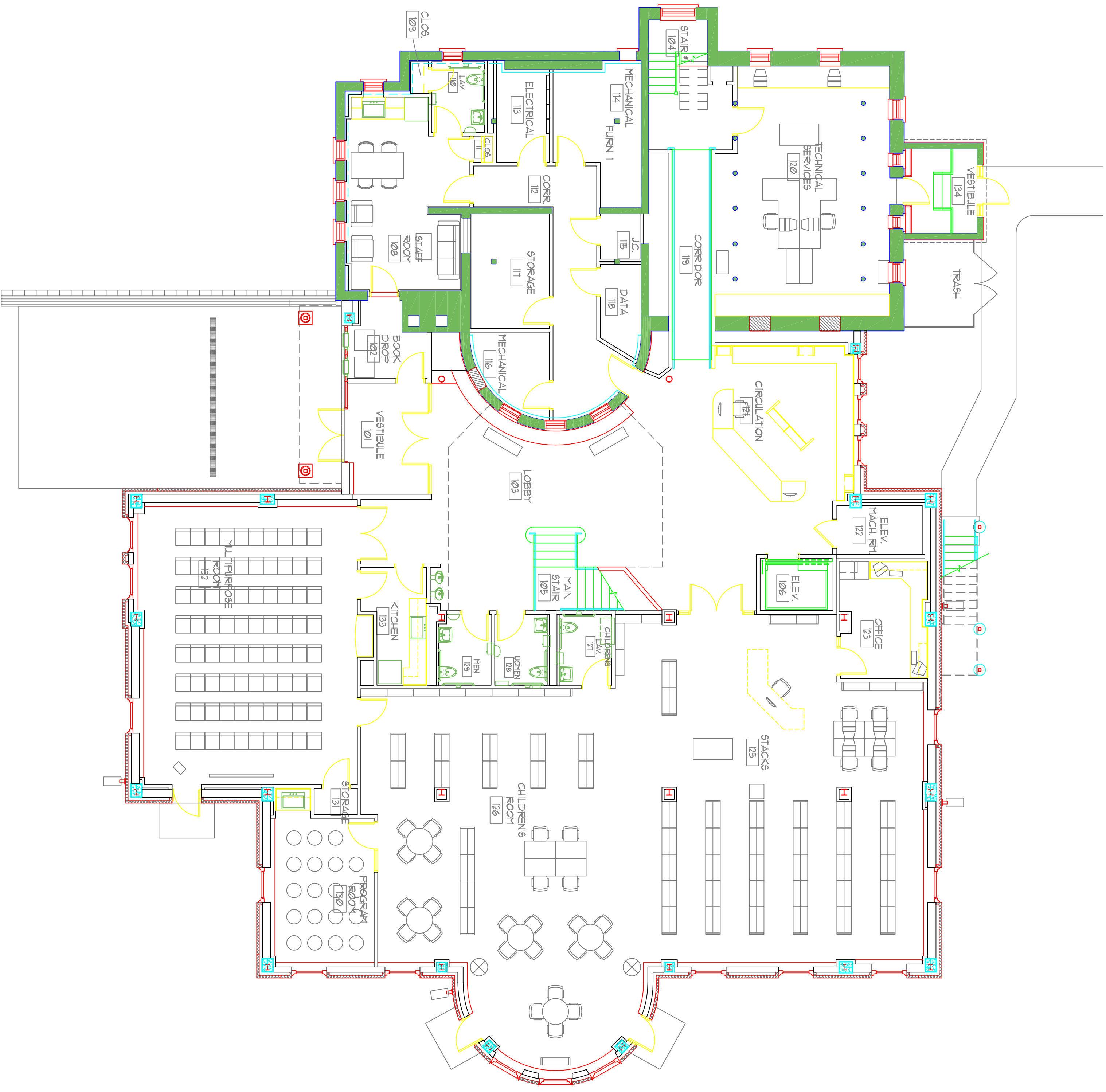
GROUND FLOOR PLAN SCALE: 1/8" = 1'-0"
